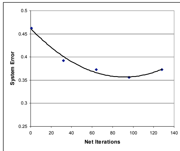
Fig. 4. Three layer neural network: iterations taken to converge on correct detection, where the effect of training can be seen after 64 iterations.
