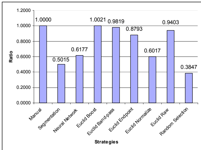
Fig. 5. Detection ratio is determined by the number of songs manually counted (488) divided by the songs detected by the strategy used.
