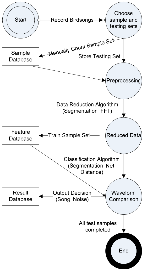
Fig. 1. The data reduction model.
